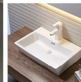
A477 Size: 605x425x130mm
