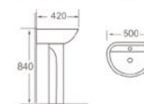
B02 Basin with pedestal Size: 500x420x840mm
