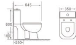
3004 Washdown two-piece toilet Size: 645x350x800mm S-trap: 250mm Roughing-in P-trap: 180mm Roughing-in
