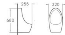
6003 Wall hung urinal Size: 320x255x680mm Fixing to wall with back
