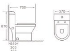
A2201 Siphonic / Washdown one-piece toilet Size: 700x370x810mm S-trap: 250/300/400mm Roughing-in P-trap: 180mm Roughing-in
