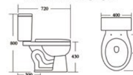
2139 Siphon two-piece toilet Size:720x400x800mm S-trap:300mm Roughing-in
