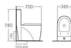
A2022 Washdown one-piece toilet Size: 700x385x780mm S-trap: 250/300mm Roughing-in
