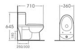
A3004LT Washdown one-piece toilet Size: 710x360x645mm P-trap: 180mm Roughing-in S-trap: 100/250/300mm Roughing-in
