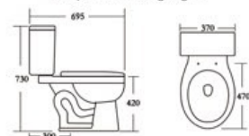
2177 Siphon two-piece toilet Size:695x370x730mm S-trap:300mm Roughing-in
