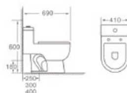
A2114 Siphonic one-piece toilet Size: 690x410x600mm S-trap: 250/300/400mm Roughing-in
