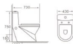
A2389 Washdown one-piece toilet Size: 730x430x750mm S-trap: 250mm Roughing-in P-trap: 180mm Roughing-in
