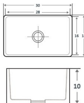
OVS-3018S 30inch single bowl ceramic kitchen sink Size:30"x18"x10"
