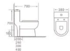
A2347 Siphonic / Washdown one-piece toilet Size: 700x380x700mm S-trap: 250/300/400mm Roughing-in P-trap: 180mm Roughing-in
