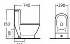
A2029 Washdown one-piece toilet Size: 740x390x850mm P-trap: 180mm Roughing-in S-trap: 300mm Roughing-in
