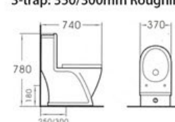
A2004 Washdown one-piece toilet Size: 740x370x780mm P-trap: 180mm Roughing-in S-trap: 350/300mm Roughing-in
