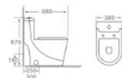
A2208 Washdown one-piece toilet Size: 680x380x670mm S-trap: 250/300/400mm Roughing-in P-trap: 180mm Roughing-in
