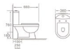
2082 Washdown two-piece toilet Size: 660x360x760mm S-trap: 100/250/300mm Roughing-in P-trap: 180mm Roughing-in
