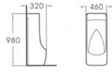
6010 Floor standing urinal Size: 460x320x980mm Fixing to wall with back
