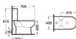
2502 Washdown two-piece closet Size: 700x400x810mm S-trap: 250mm Roughing-in P-trap: 180mm Roughing-in
