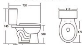
2138 Siphon two-piece toilet Size:720x410x745mm S-trap:300mm Roughing-in
