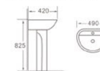
B28 Basin with pedestal Size: 490x420x825mm
