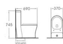
A2019 Siphonic one-piece toilet Size: 690x370x745mm S-trap: 300/400mm Roughing-in
