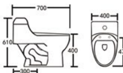
JX-820 Ceramic name:Siphonic One-piece Closet Size:700x400x610mm S-trap:300mm Roughing-in
