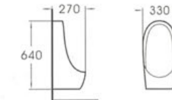
6004 Wall hung urinal Size: 330x270x640mm Fixing to wall with back
