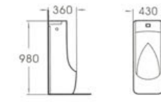
6001 Floor standing urinal Size: 430x360x980mm Fixing to wall with back
