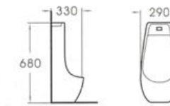
6005 Wall hung urinal Size: 290x330x680mm Fixing to wall with back
