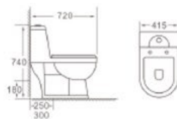
A2111B Washdown one-piece toilet Size: 720x415x740mm S-trap: 250/300/400mm Roughing-in P-trap: 180mm Roughing-in
