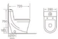
A2209 Washdown one-piece toilet Size: 720x390x750mm S-trap: 250/300mm Roughing-in P-trap: 180mm Roughing-in
