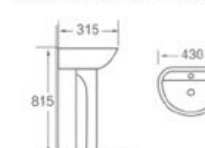
B81 Basin with pedestal Size: 430x315x815mm
