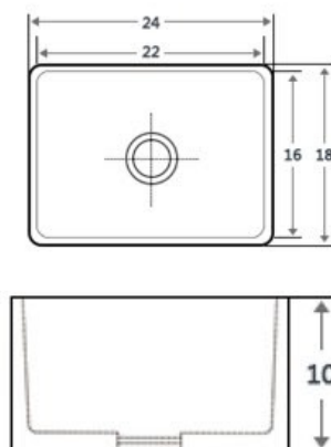
OVS-2418S 24inch single bowl ceramic kitchen sink Size:24"x18"x10"
