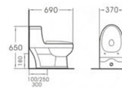
A2031 Washdown one-piece toilet Size: 690x370x650mm P-trap: 180mm Roughing-in S-trap: 100/250/300mm Roughing-in
