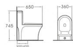
A2026 Siphonic one-piece toilet Size: 650x360x745mm S-trap: 300/400mm Roughing-in
