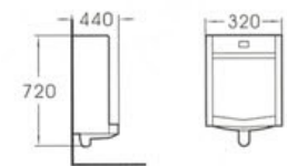
6008 Wall hung urinal Size: 320x440x720mm Fixing to wall with back
