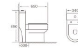
A2334 Siphonic one-piece toilet Size: 650x340x690mm S-trap: 300/400mm Roughing-in
