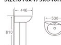
A7156 Basin with pedestal Size: 610x475x840mm
