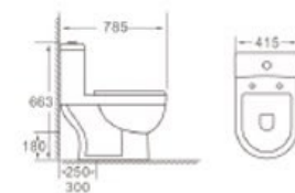
A2388 Washdown one-piece toilet Size: 785x415x663mm S-trap: 250/300mm Roughing-in P-trap: 180mm Roughing-in
