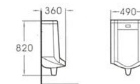
6007 Wall hung urinal Size: 490x360x820mm Fixing to wall with back
