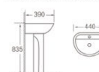
B65 Basin with pedestal Size: 440x390x835mm
