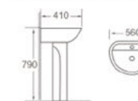
B52 Basin with pedestal Size: 560x410x790mm
