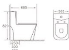
A2205 Siphonic / Washdown one-piece toilet Size: 685x385x820mm S-trap: 250mm Roughing-in
