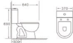
2081 Siphonice two-piece toilet Size: 640x370x690mm S-trap: 300mm Roughing-in
