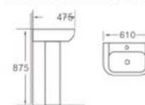
A7103 Basin with pedestal Size: 610x475x875mm
