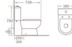
3007 Washdown two-piece toilet Size: 700x380x790mm S-trap: 250mm Roughing-in P-trap: 180mm Roughing-in
