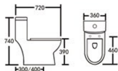
JX-843 Ceramic name:Siphonic One-piece Closet Size:720x360x740mm S-trap:300/400mm Roughing-in
