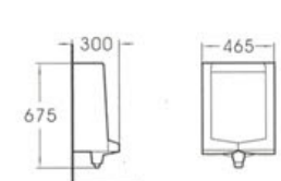
6006 Wall hung urinal Size: 465x300x675mm Fixing to wall with back
