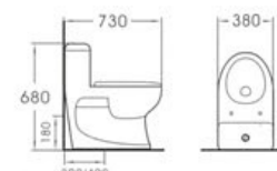
A2030 Washdown one-piece toilet Size: 730x380x680mm P-trap: 180mm Roughing-in S-trap: 300/400mm Roughing-in
